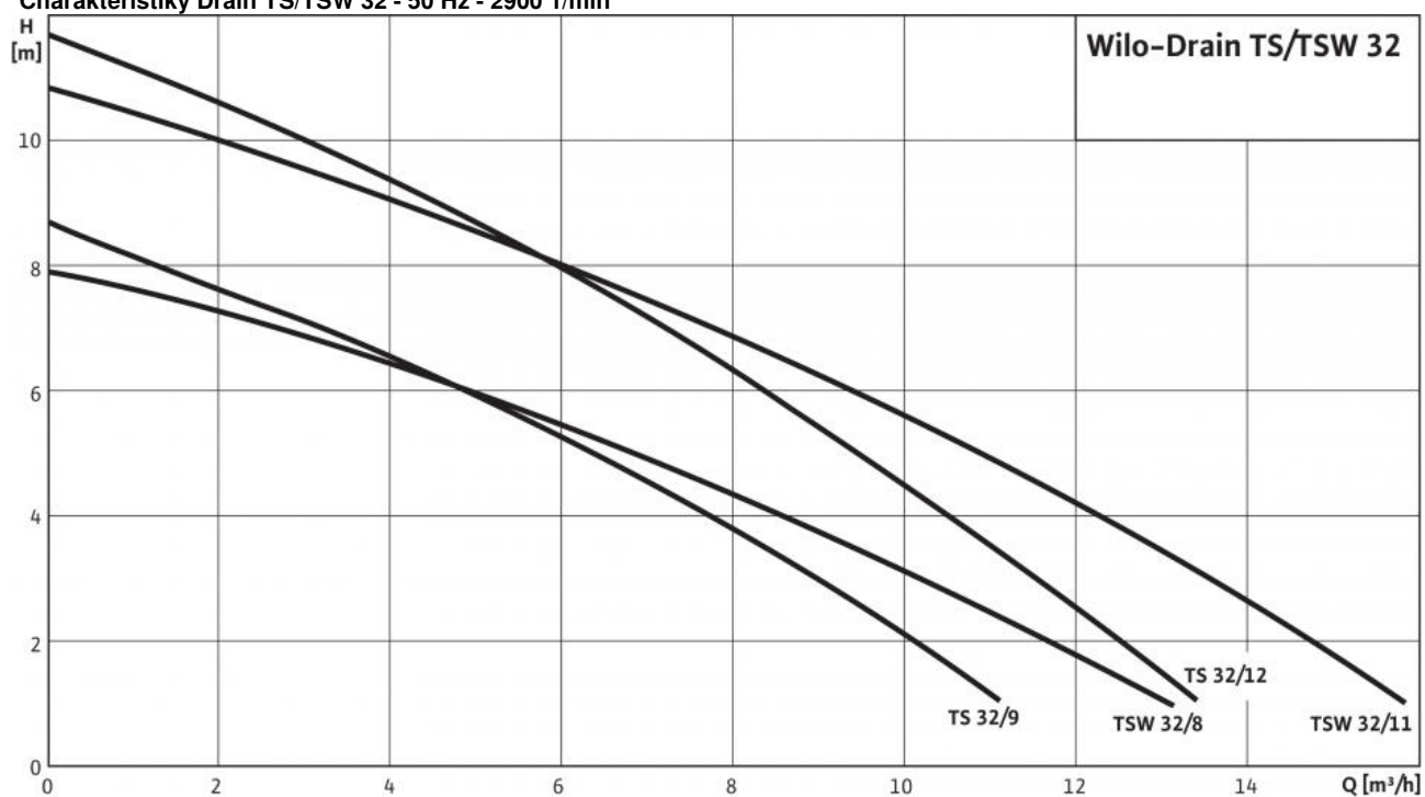
Charakteristiky Drain TS/TSW 32 - 50 Hz - 2900 1/min
